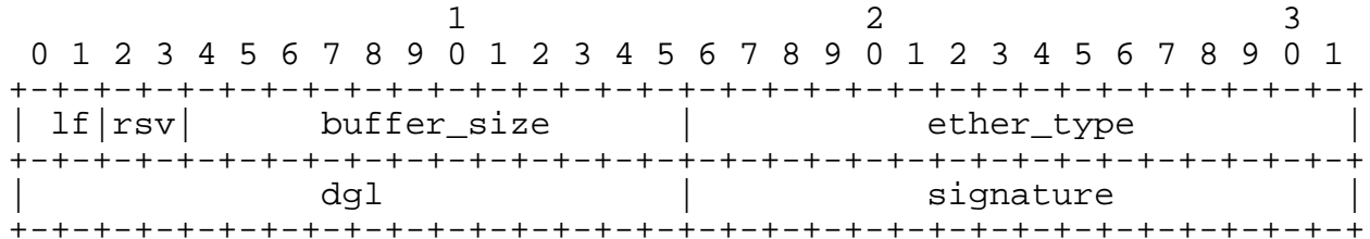
Figure 3 - First fragment encapsulation header format
