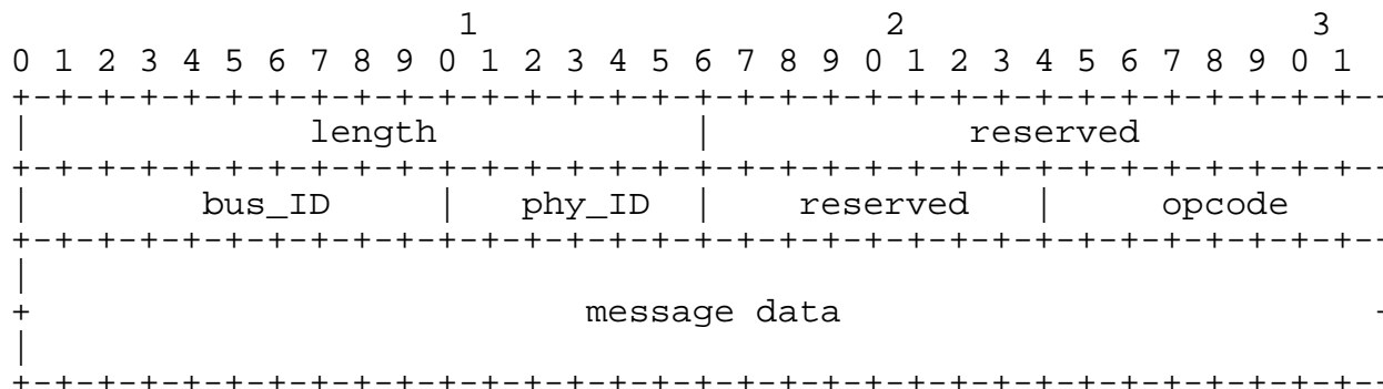
Figure 6 - MCAP message format
