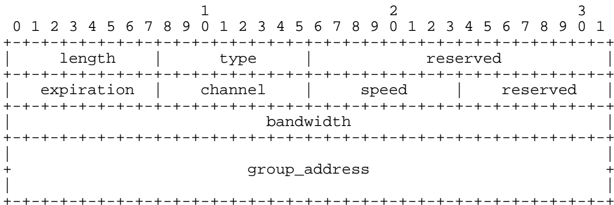
Figure 7 - MCAP group address descriptor format
