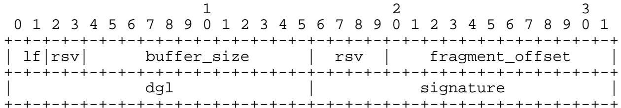
Figure 4 - Subsequent fragment(s) encapsulation header format
