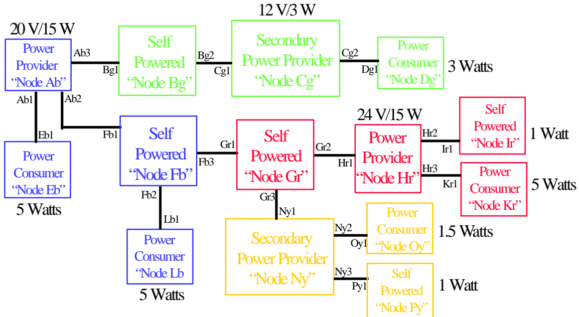
Figure 6-16 – Example Suspend/Resume Domain Topology
