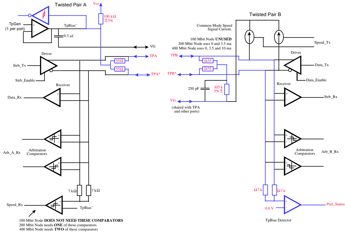
Figure 6-12 – Cable media signal interface configuration with Suspend Connection Circuitry
