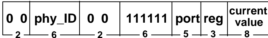
Figure 6-14 – PHY-Access Response Packet
