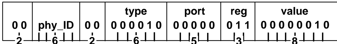
Figure 6-15 – Extended PHY Packet of type “Resume”
